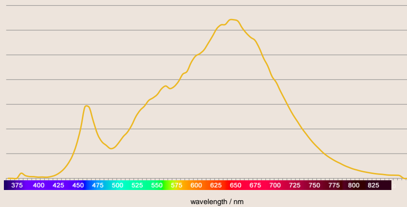
SPECTRAL POWER DISTRIBUTION OF LEDON 10W DOWNLIGHT
